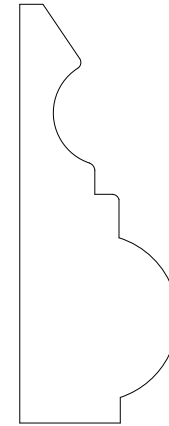
FBC526 13/16" X 2-3/16"
