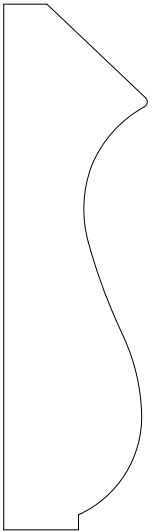
FBC465 3/4" X 2-3/4"
