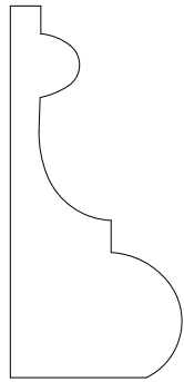
FBC438 13/16" X 1-3/4"
