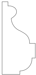
FBC466 3/4" X 1-9/16"
