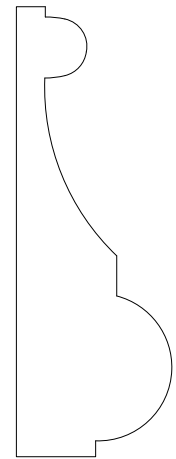
FBC330 13/16" X 2-3/8"
