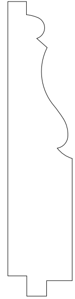
FBC326 3/4" X 3-1/8"
