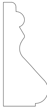
FBC319 3/4" X 1-3/4"
