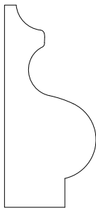
FBC302 11/16" X 1-1/2"
