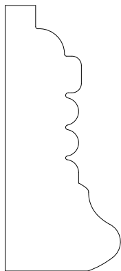
FBC135 7/8" X 2-1/16"
