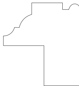
FBB184 1-9/16" X 1-1/2"
